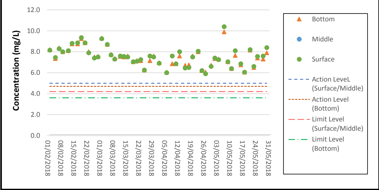
DO Concentrations at Station SR4(N) (Mid Ebb)
