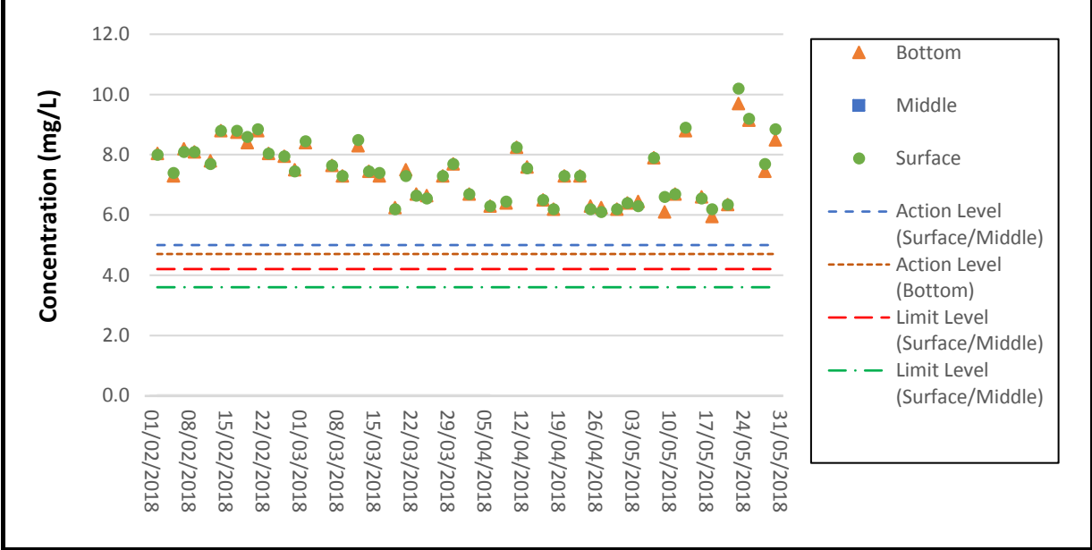
DO Concentrations at Station SR4(N) (Mid Flood)
