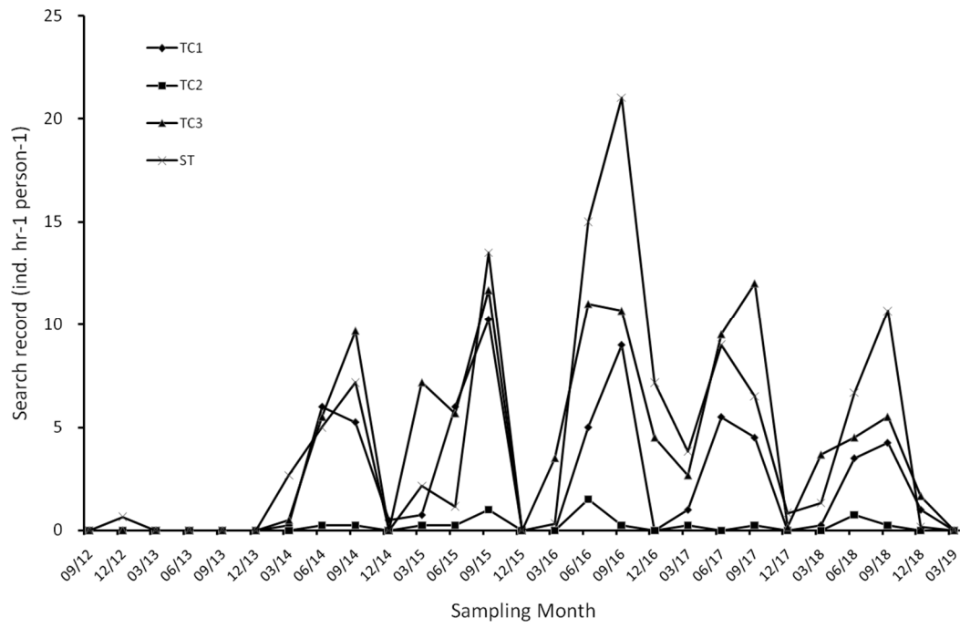
Figure 3.5 (Cont'd). Changes of number of individuals mean prosomal width and search record of horseshoe crab Carcinoscorpius rotundicauda in every sampling zone along the sampling months
