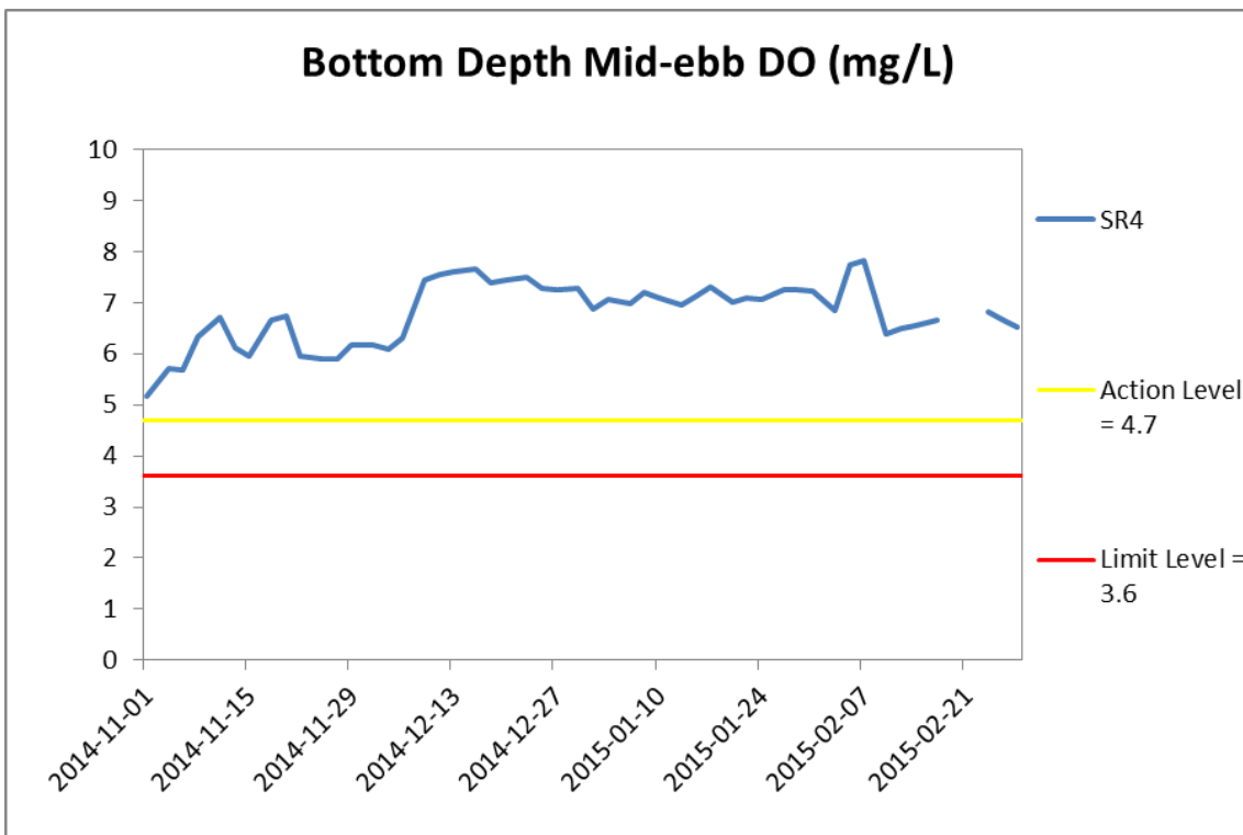
Figure H15 Impact Monitoring - Mean Level of Dissolved Oxygen (mg/L) in bottom waters during mid-ebb tide between 1 November 2014 and 28 February 2015 at IS8 and SR4.
