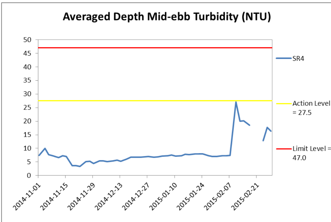
Figure H23 Impact Monitoring - Mean Level of depth-averaged Turbidity (NTU) during mid-ebb tide between 1 November 2014 and 28 February 2015 at IS8 and SR4.
