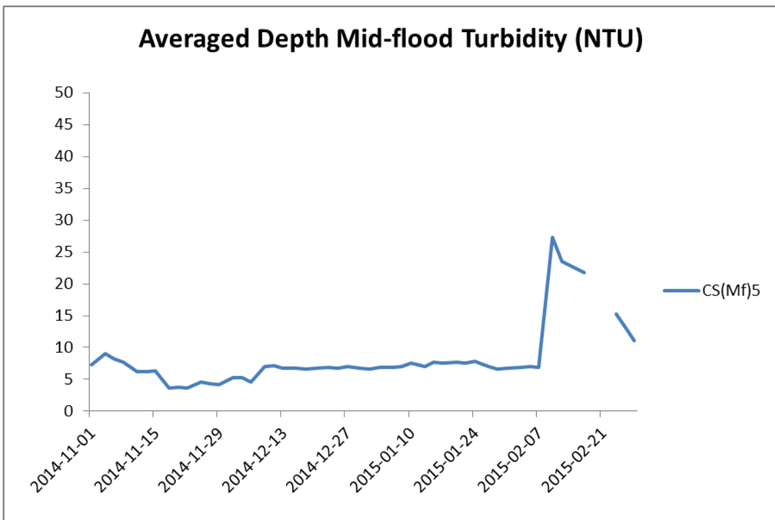
Figure H25 Impact Monitoring - Mean Level of depth-averaged Turbidity (NTU) during mid-flood tide between 1 November 2014 and 28 February 2015 at CS(Mf)3 and CS(MF)5.
