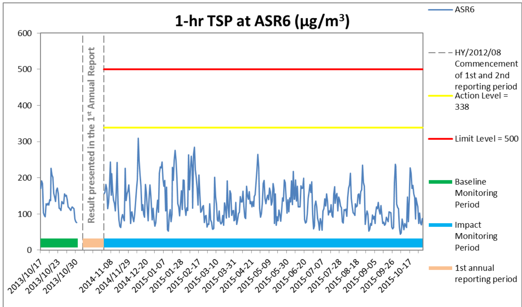
Figure D.2 Baseline & Impact Monitoring - 1-hour Total Suspended Particulates ( \mu\text{g}/\text{m}^3 ) at AQMS2/ASR6 between 17 October 2013 and 31 October 2015 during Baseline & Impact Monitoring period. Weather condition within the reporting period varied between sunny to rainy. The overall monitoring results were not affected by weather conditions. Major land-based construction activities included: Excavation for North Launching Shaft, Diaphragm Wall Construction, Land-based Sheet Piling Works, Box Culvert Extension, Construction of temporary access, TBM Platform Construction & Start-up of TBM. Ref: 0212330_Impact AQM graphs_2ndAnnual_REV a.xlsx
